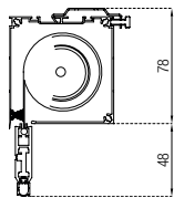
Fondale 11x41 Bottom rail 11x41
