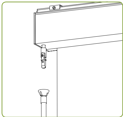
Asta asportabile Removable crank rod
